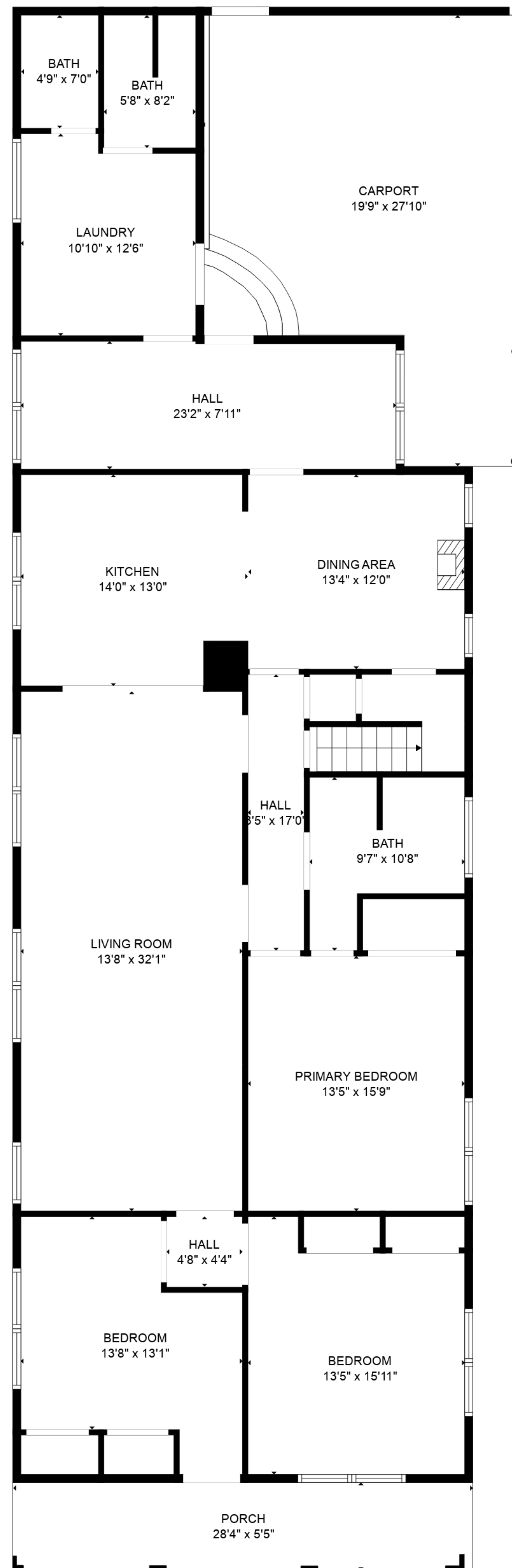
FLOOR 1
