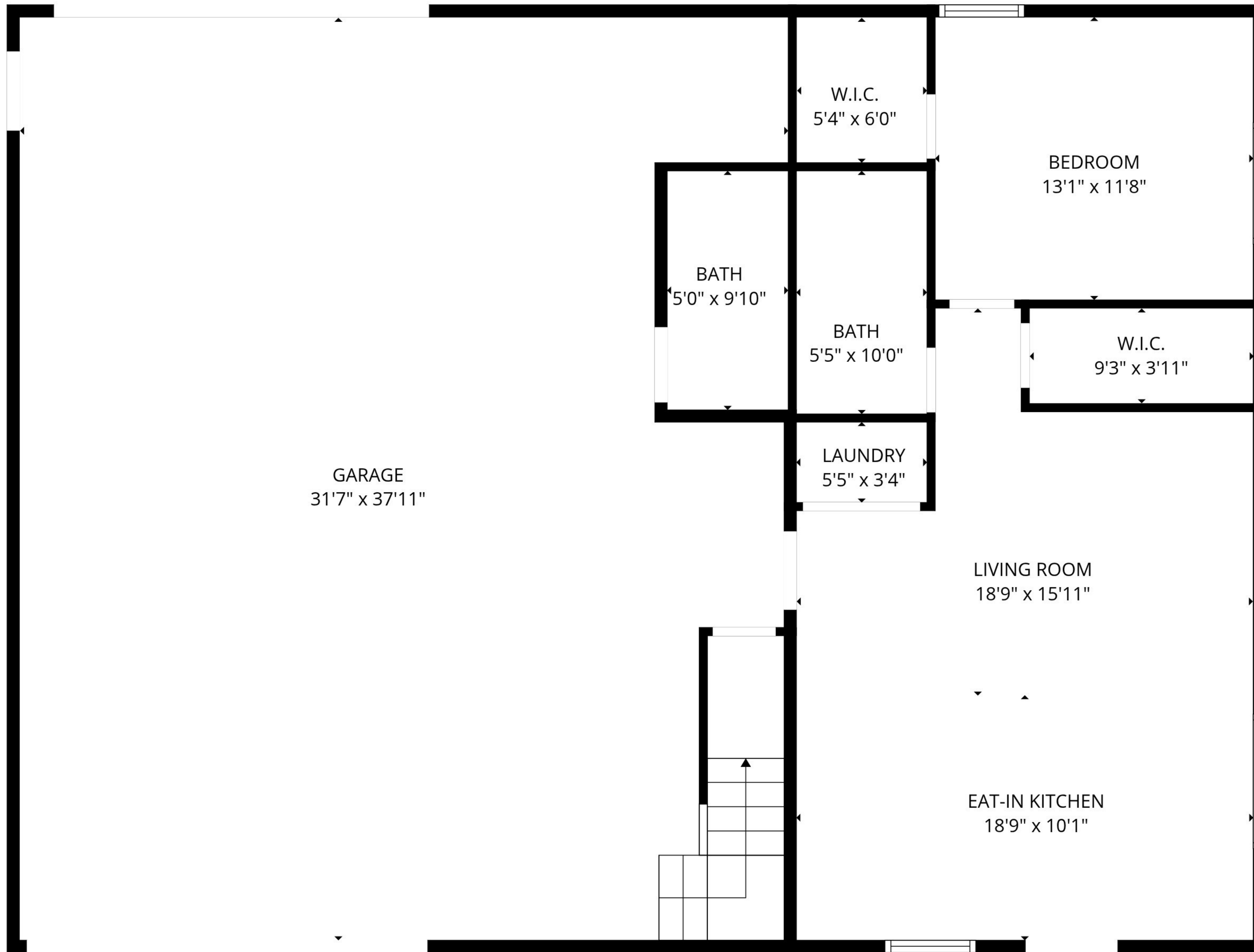
1st floor
