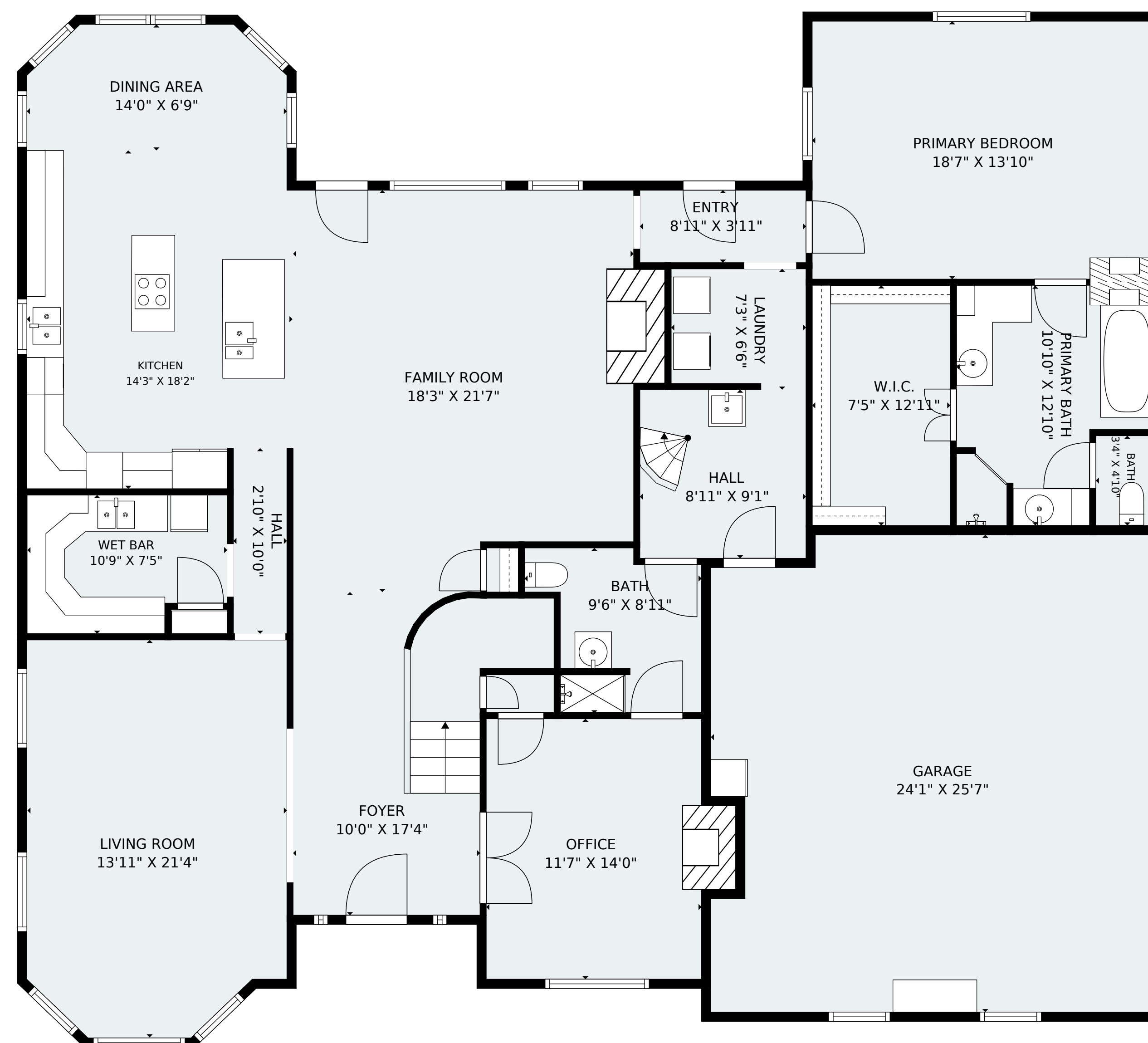
1ST FLOOR
