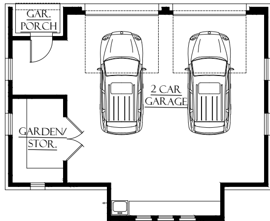
DETACHED GARAGE FLOOR PLAN
