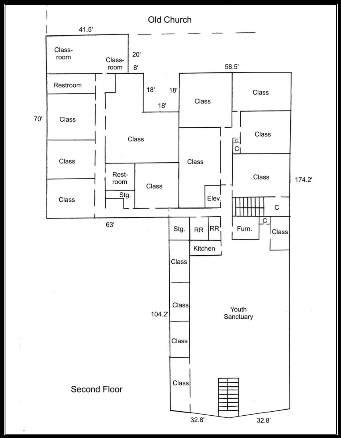
Floor Plan – Second Floor
