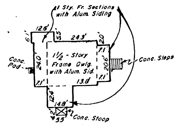
DWELLING DETAIL SCALE: 1" = 30'
