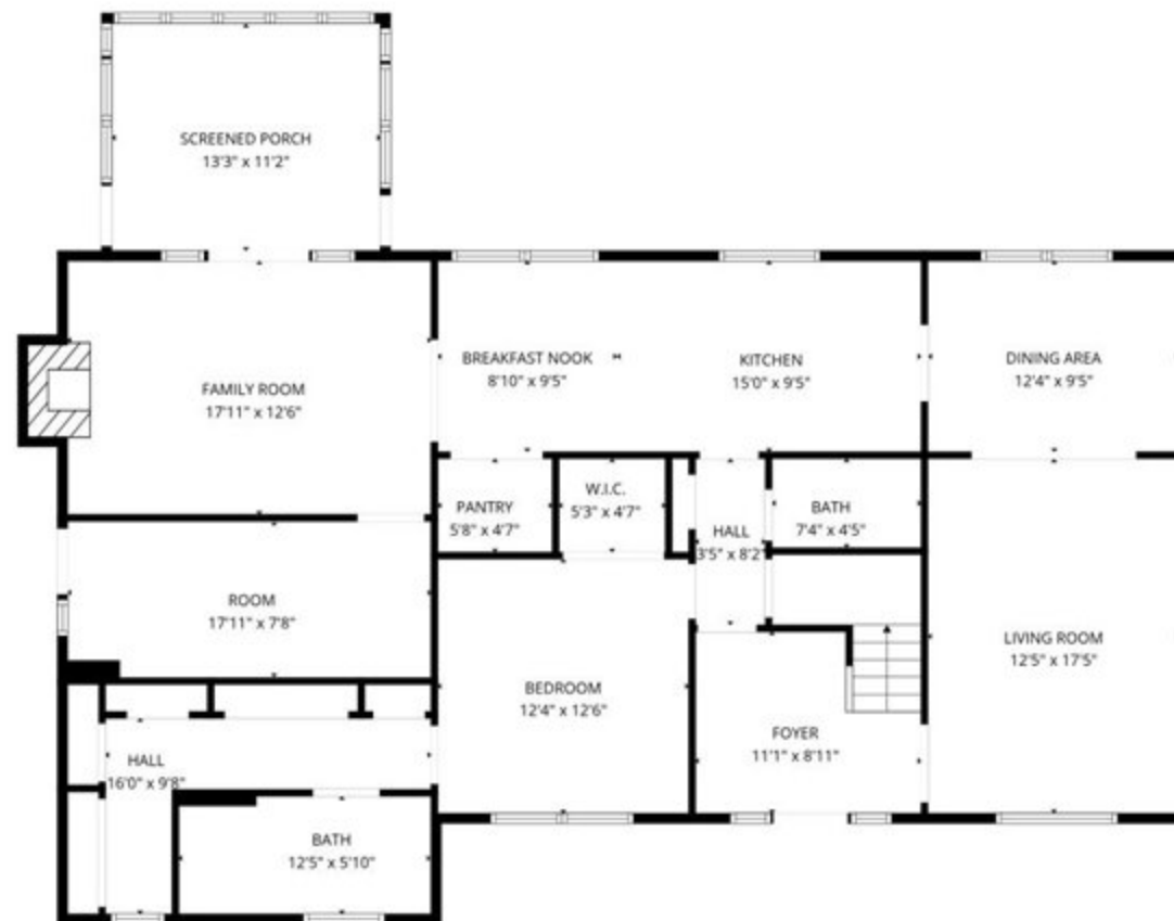
2nd floor
