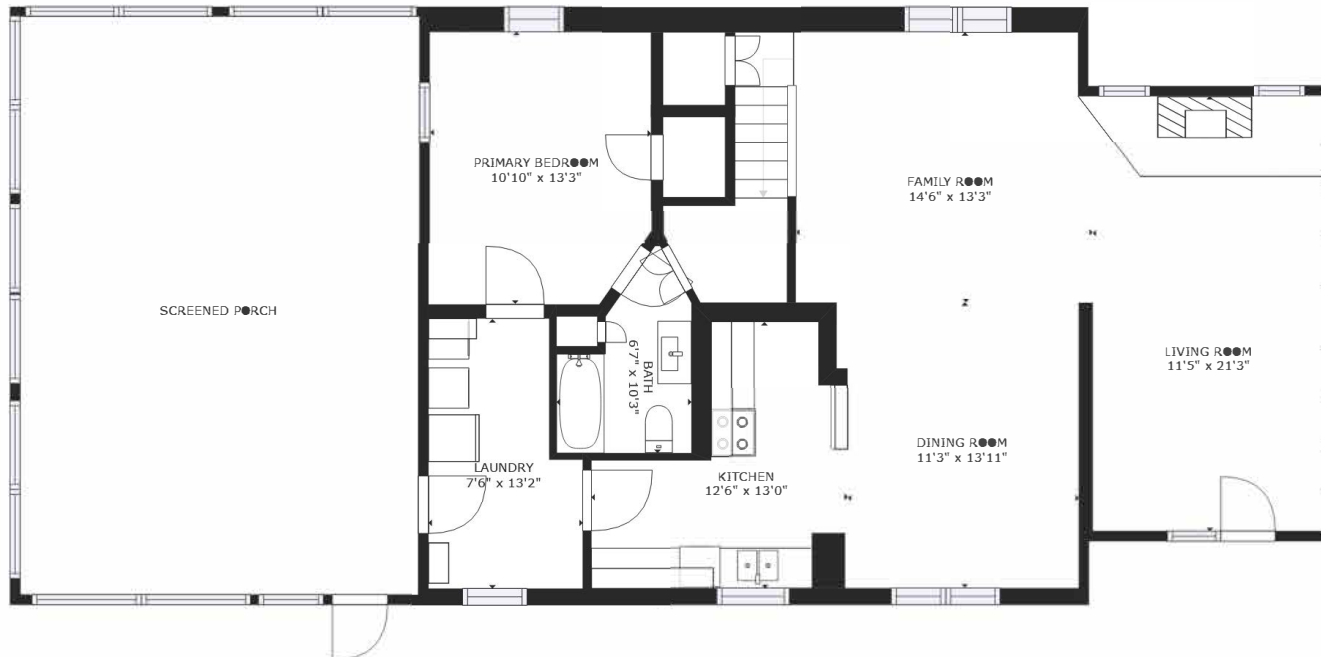
FLOOR 1
